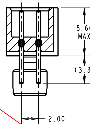
SECTION Z-Z
